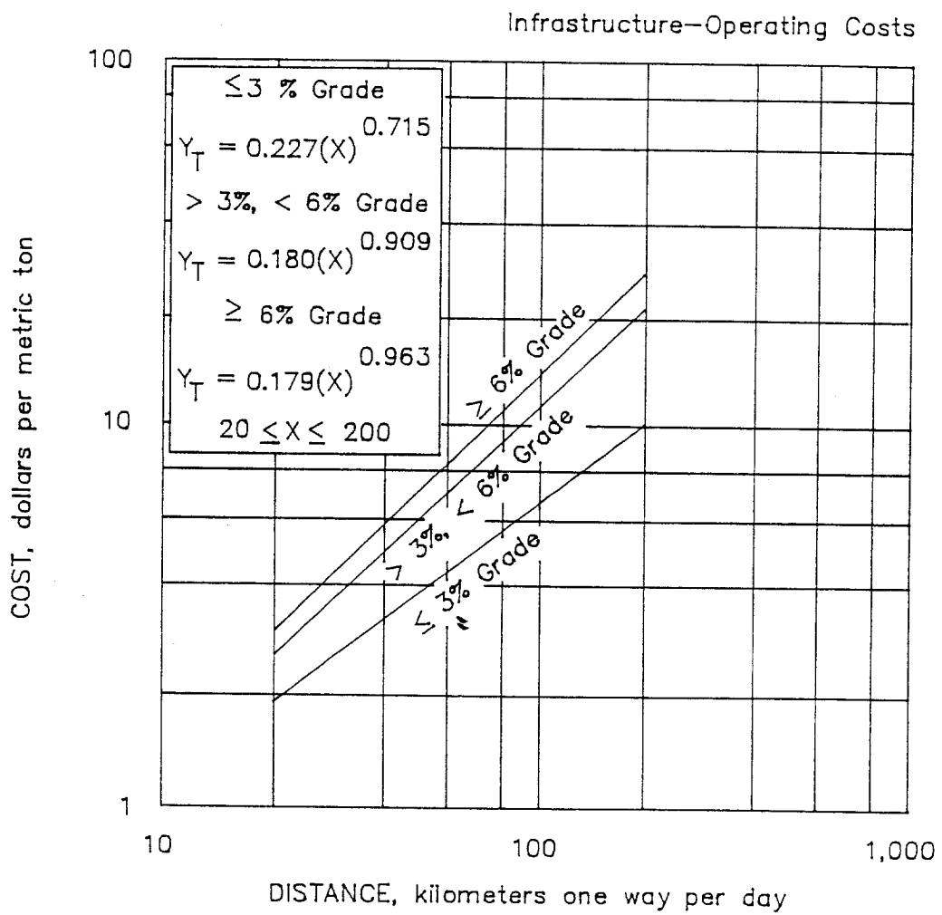
9.1.4.6. Long distance truck haulage
